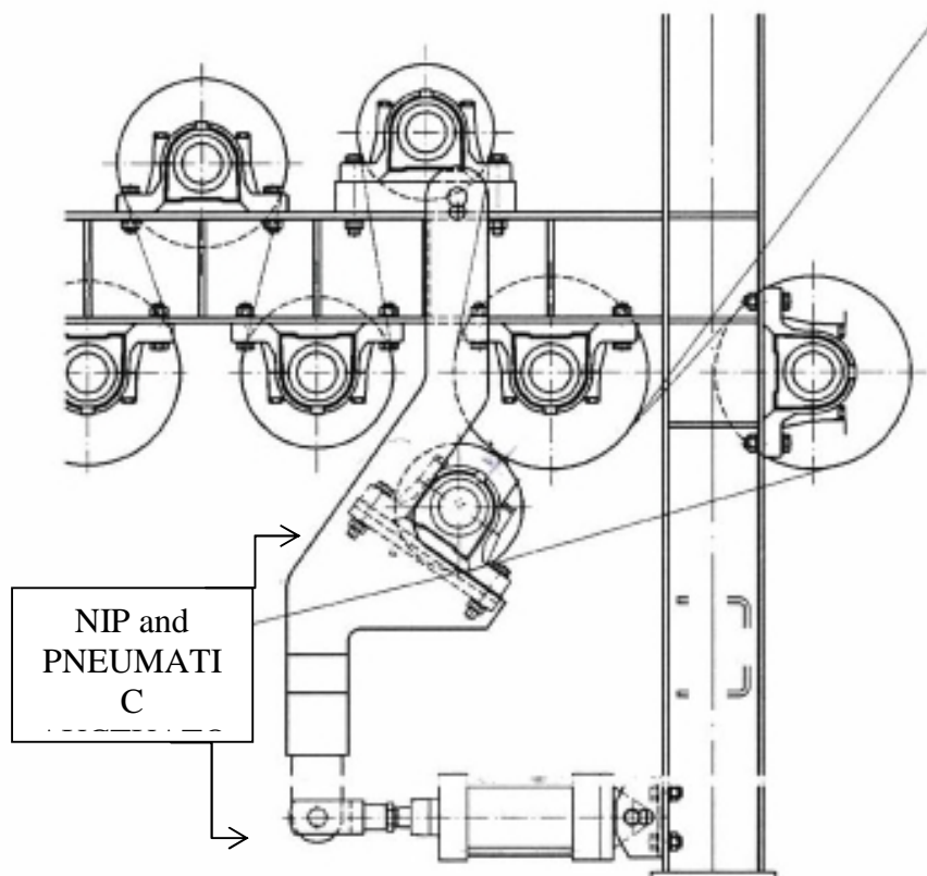
Figure 1: Belt Filter Press Nip
