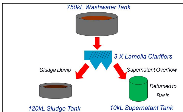
Figure 1: Woodglen water treatment plant washwater system
