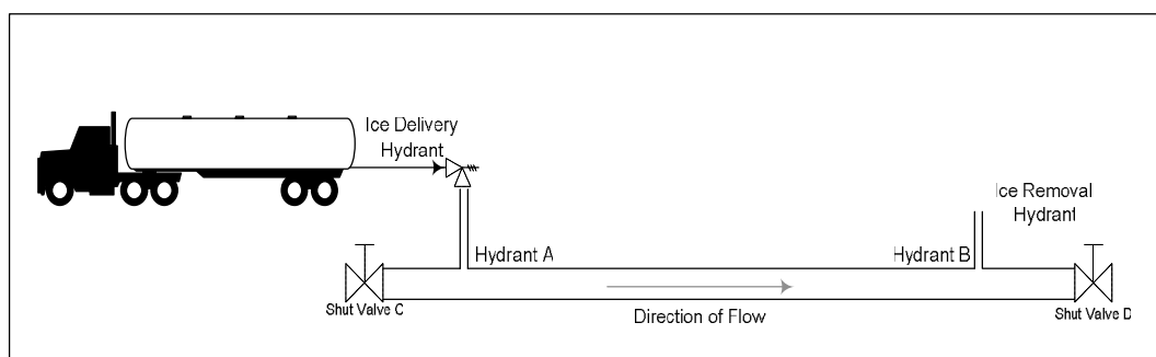
Figure 3: Schematic of ice pigging process
