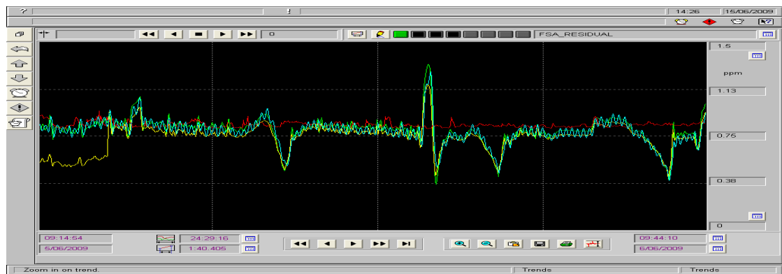
Figure 1: SCADA trend showing a uniform trend from the trial meters. Note the yellow line of the prominent analyser before and after a calibration.
