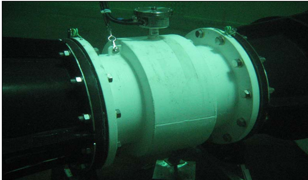
Figure 1: Siemens flow meter mounted between tapered HDPE pipe work.
