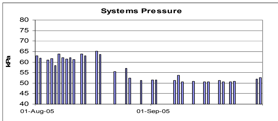
Figure 6: Graph showing backpressure changes before and after diffuser cleaning
